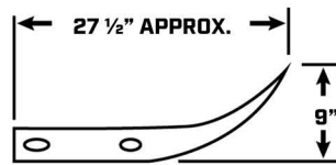
END SECTION (FLARED)
